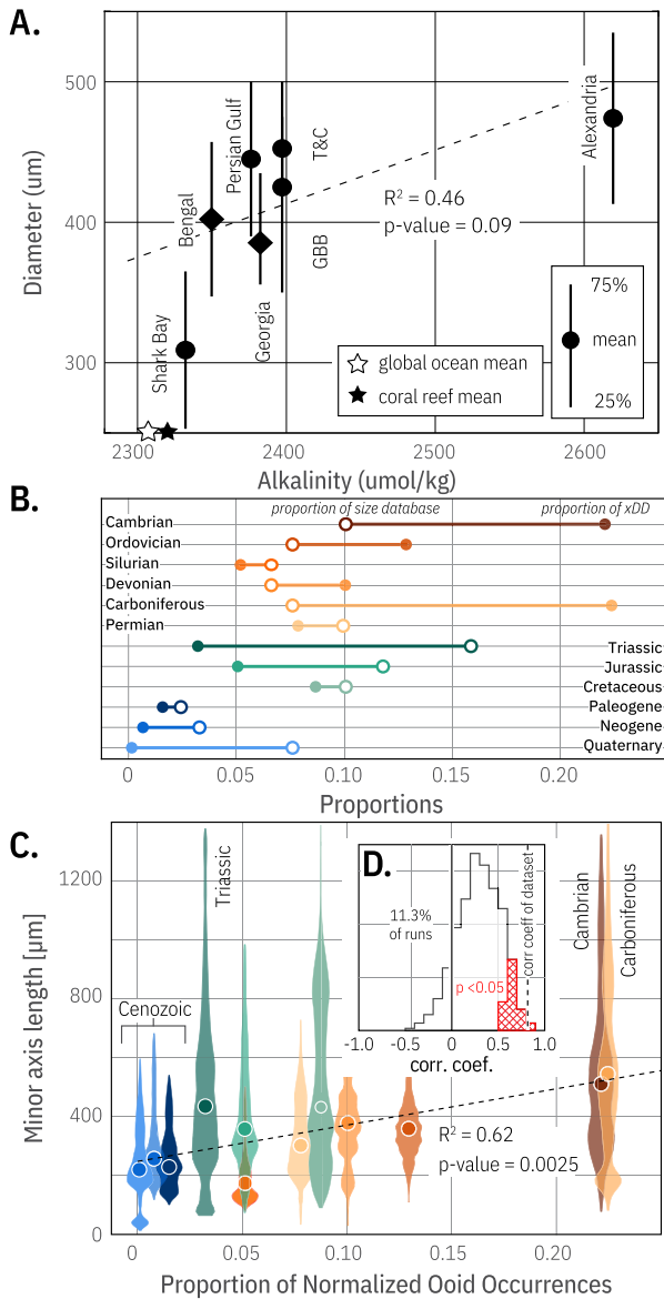
Fig. 8. Higher alkalinity may result in larger ooid sizes in the modern and Phanerozoic. A. Diameter of ooids as a function the total alkalinity of the source waters. The total alkalinity of source waters is from the Global Data Analysis Project (Key et al., 2004). Ooid sizes from Turks and Caicos (Trower et al., 2018), The Bahamas, and Shark Bay were measured with a camsizer. Ooid sizes from the Persian Gulf are from Abu Dhabi Island and measured with a sieve (Loreau and Purser, 1973). Measurements from Alexandria Beach, Egypt were made on photomicrographs from (El-Sammak and Tucker, 2002). Depending on the composition of seawater, as alkalinity increases, the increases in saturation state slow down because of reduced ion activity (Zeebe and Tyrrell, 2019). B. To address potential bias from uneven sampling in the database of ooid sizes (Koeshidayatullah et al., 2022), we utilized a resampling approach that adjusted the size database to match the proportions found in the xDD database, using the same weighting scheme as illustrated in (Fig. 7A). C. After resampling, we find that there is a statistically significant correlation ( p = 0.0025 ) between the abundance of ooids and the median minor axis length of ooids from that period. D. To evaluate if the correlation is robust, we ran 1000 simulations, each time randomly selecting locations for each period and drawing ooids from these locations. We calculate the correlation coefficient between the median size and proportion of normalized ooid occurrences. We get a range of correlation coefficients, but only strong, positive correlations have statistically significant p -values.
