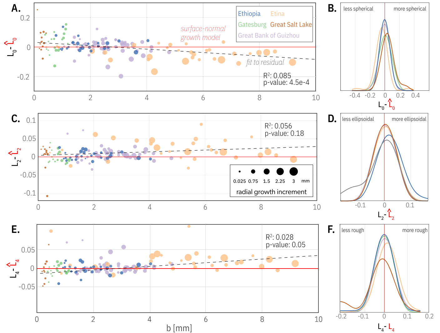
Fig. 5. The comparison of measured ooid growth to the surface-normal growth model. A. Surface normal growth alone explains 92.7% of the change in L_0 . B. Mean of all residuals is -0.01. C. Surface normal growth alone explains 82.7% of the change in L_2 . Positive values indicate long axes becoming longer than surface-normal growth predicts. Negative values indicate short axes becoming longer than surface-normal growth predicts. D. The residuals of the giant ooid samples have means that are very slightly positive, which suggest that surface normal growth does a good job explaining the change in shape, but there is a small contribution from rolling or sliding. The mean of the Gatesburg residual is very slightly negative, suggesting it is becoming a bit more spherical than surface-normal growth predicts. E. Surface normal growth alone explains ~ 55% of the change in L_4 . Positive values represent more bumps and unevenness in the surface texture. Negative values represent smoother surfaces. F. The mean of all residuals is centered on zero. There are a couple of outliers from the Great Bank of Guizhou, likely because many of those ooids broke leaving sharp edges susceptible to fragmentation (Fig. 3B).
